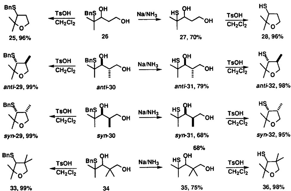
Scheme 2; Preparation and Rearrangement of 4-Benzyl sulfanyl- and 4-Sulfanyl-1,3-alkanediols
